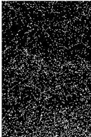
Edges (Canny)
