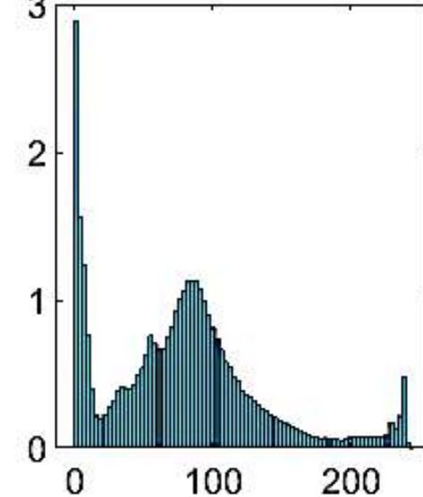
Gray Histogram
