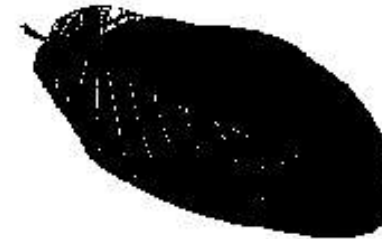
Binary
