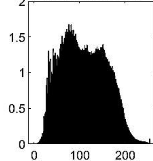
Gray Histogram
