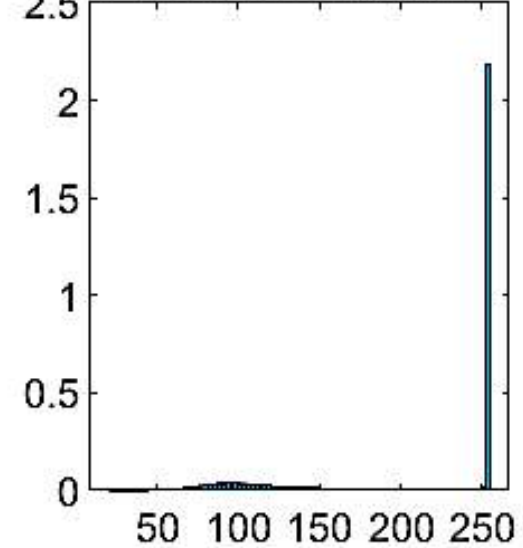
Gray Histogram
