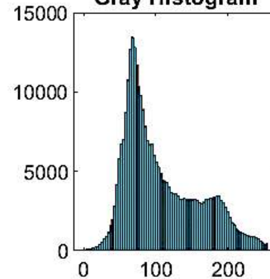
Gray Histogram
