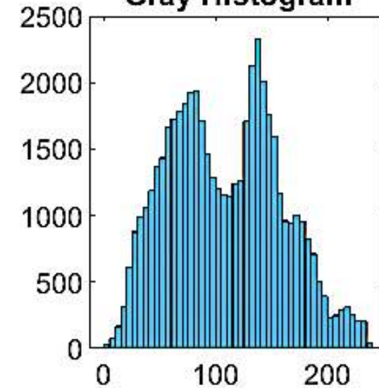
Gray Histogram
