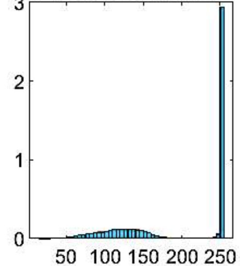
Gray Histogram
