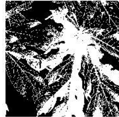
Binary
