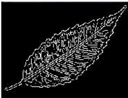
Edges (Canny)
