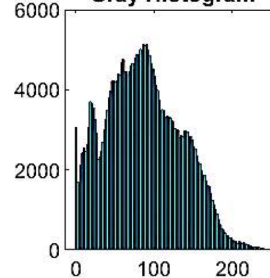
Gray Histogram
