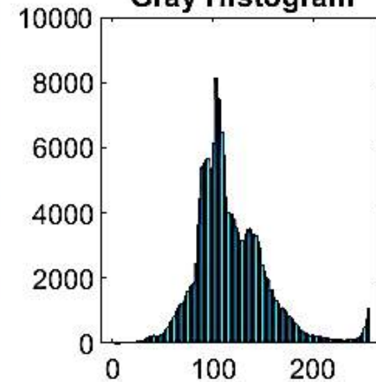
Gray Histogram
