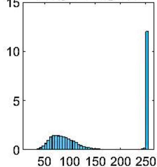
Gray Histogram
