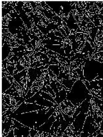
Edges (Canny)
