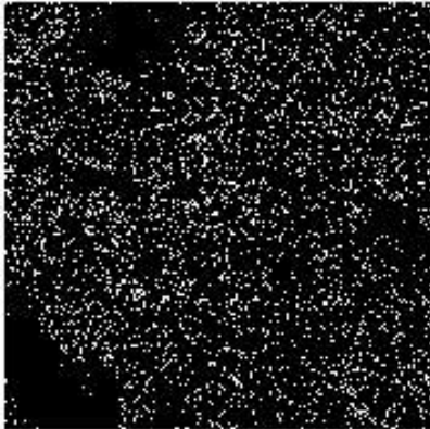
Edges (Canny)
