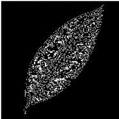
Edges (Canny)
