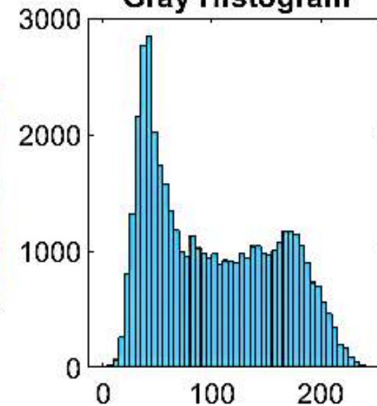
Gray Histogram
