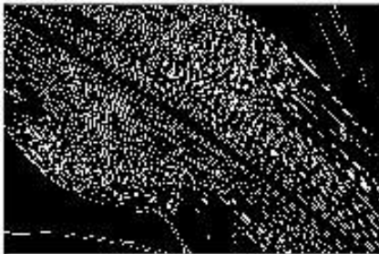
Edges (Canny)
