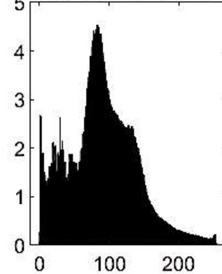
Gray Histogram
