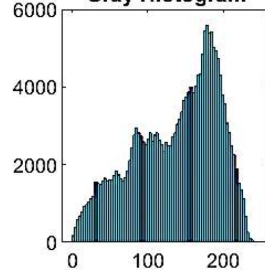
Gray Histogram
