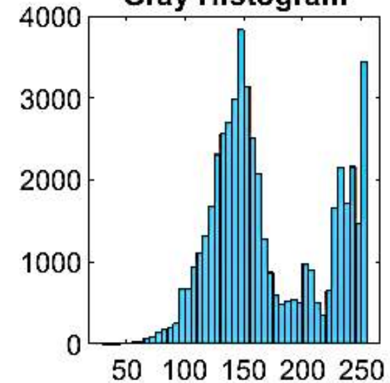
Gray Histogram
