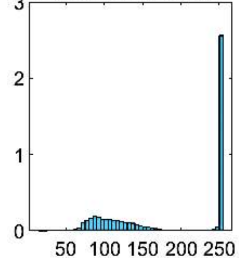
Gray Histogram
