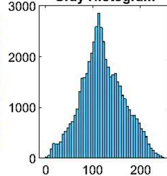
Gray Histogram
